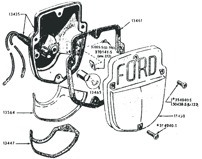
1957-1972 REAR LAMP (SHIELD TYPE)
