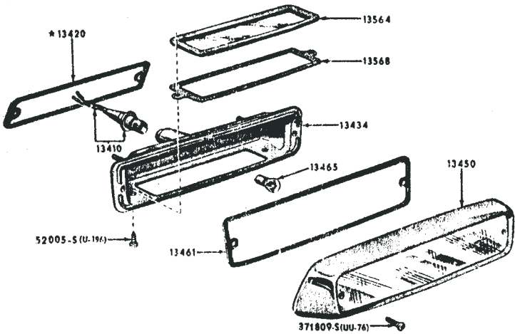
1957-1960 REAR LAMP & LICENSE PLATE F100 PANEL DELIVERY
