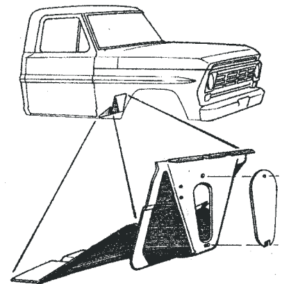
FRONT CAB MOUNT
